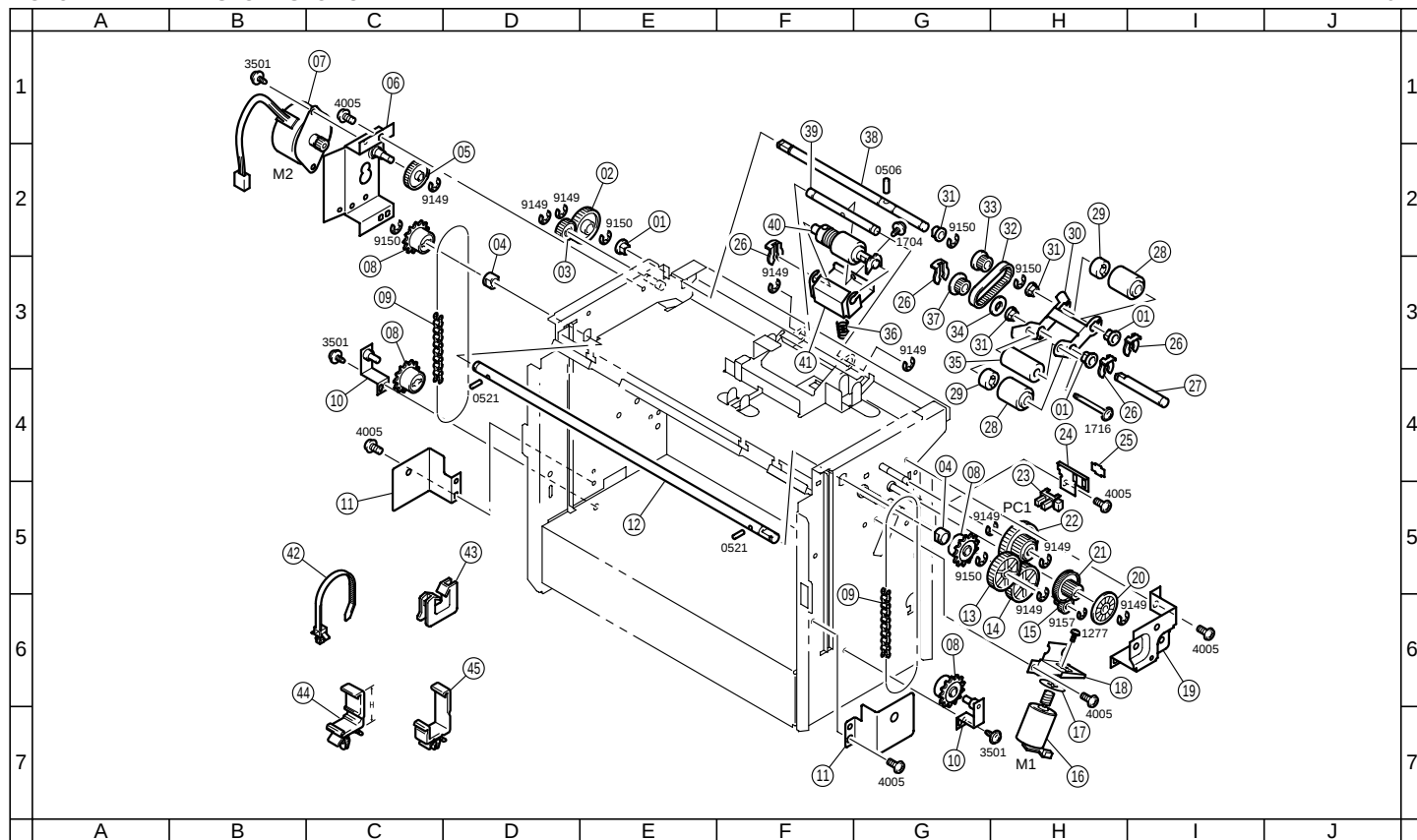
FIG. 3 PAPER TRANSPORT SECTION
