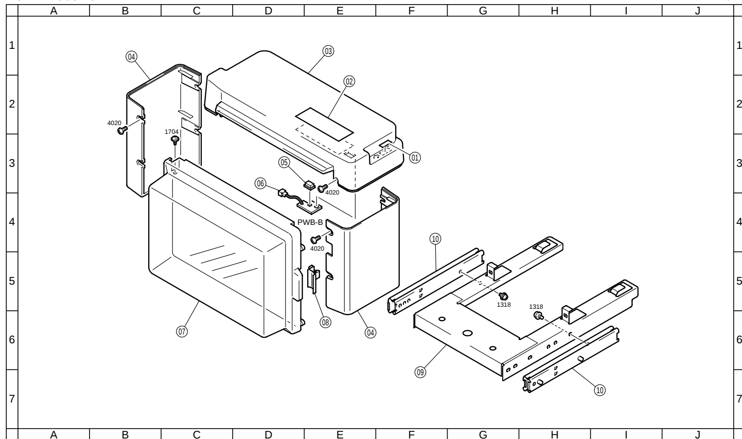
FIG. 1 HOUSING
